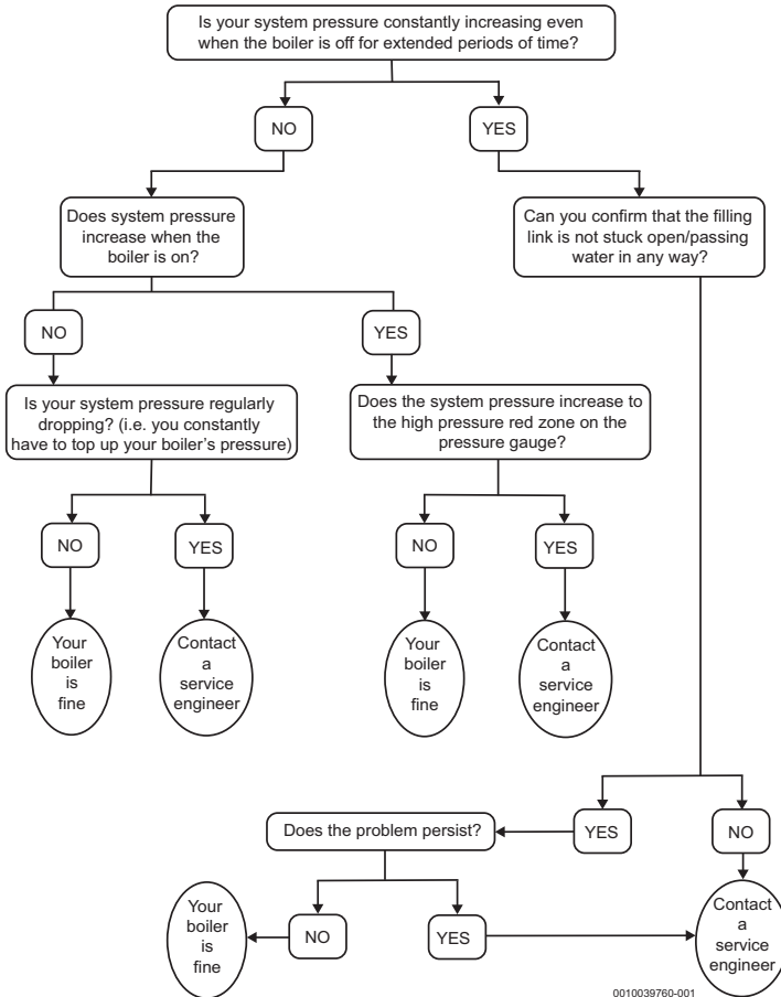
Fig. 8 System gassing trouble-shooting flow chart
